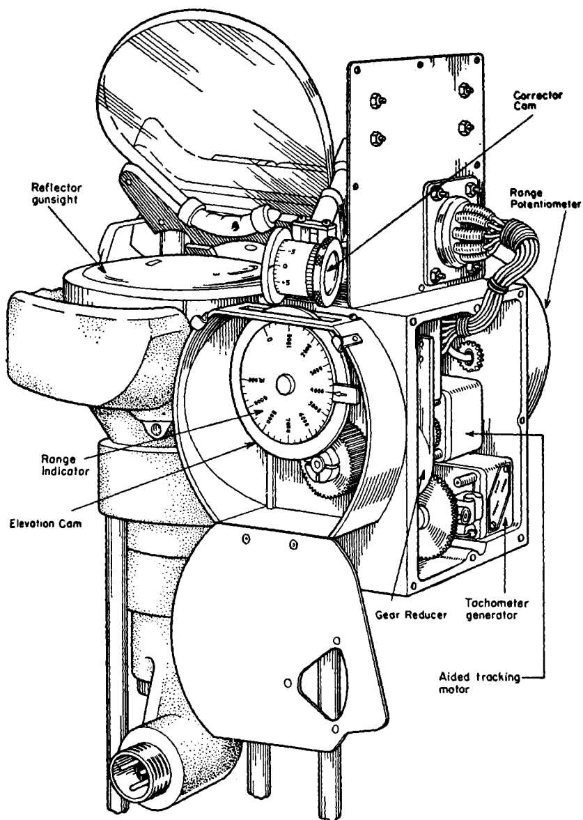
FIG. 7-48a.—Gun-sight unit of AN/APA-30.
