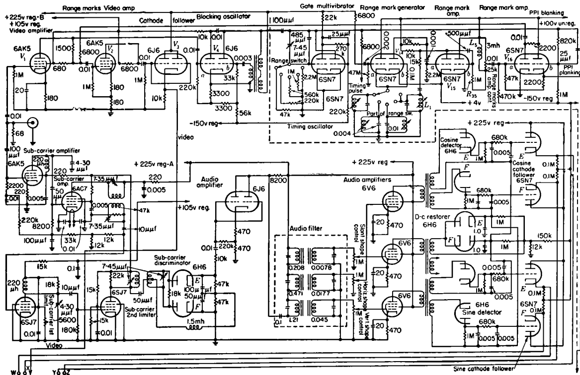
FIG. 11.35.—Separator of ARR-17 relay radar.
