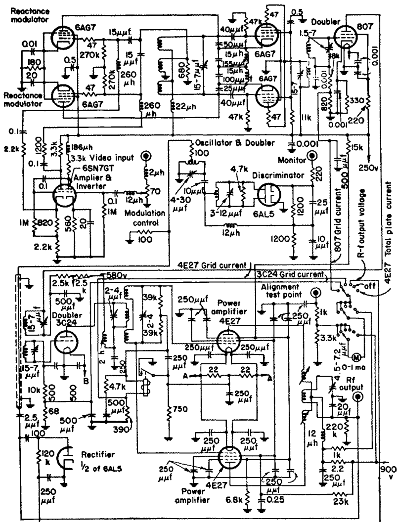
Fig. 11-33.—Transmitter of ART-18 relay radar.
