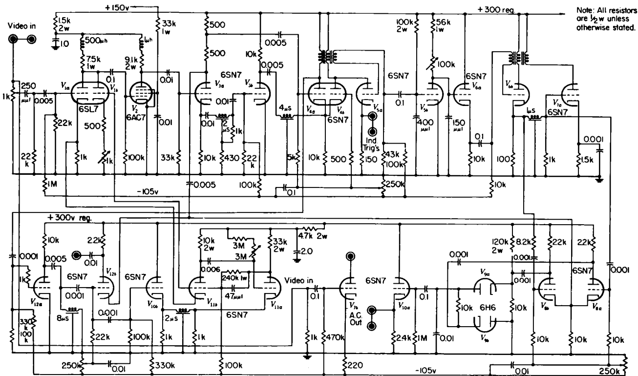
FIG. 11-27.—Decoder of simplified relay radar.
