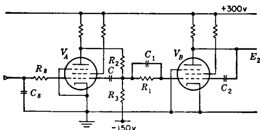
FIG. 8-19.—Actual circuit equivalent to circuit of Fig. 8-16.
