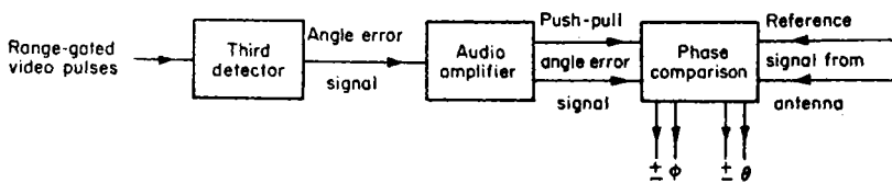
FIG. 9-32.—Block diagram of generalized angle-measuring circuit.
