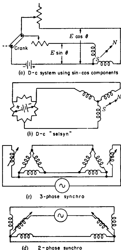
FIG. 10-2.—Devices that transmit 360^\circ rotation.
