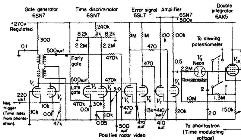
FIG. 9-39.— H_3X tracking loop.
