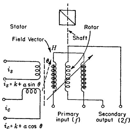
FIG. 11-16.—D-c resolver.
