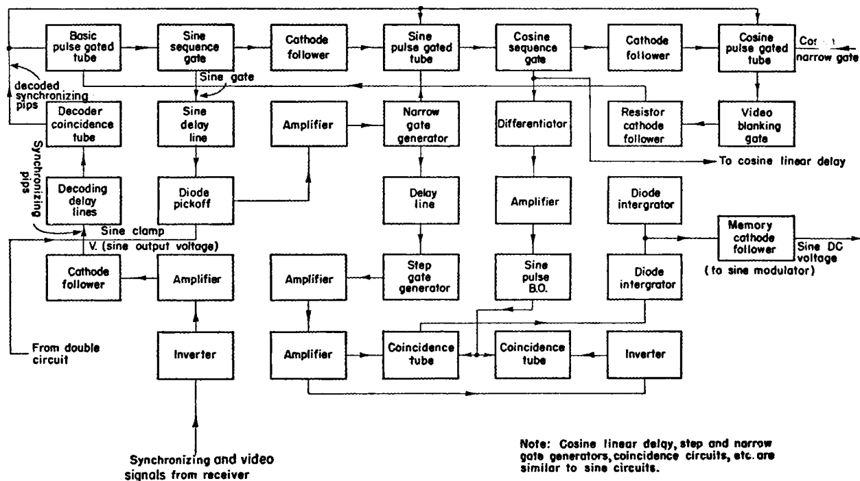
FIG. 11-8.—Input, decoding, and sine-voltage circuits.
