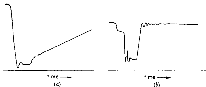
FIG. 3-2.—Voltage and current waveform in a magnetron oscillator. (a) shows the applied voltage waveform and (b) the oscillator current. The pulse duration is 10\text{ }\mu\text{sec} . In (a) the slow decay of the switching waveform is not typical of good modulator performance and could easily have been arranged to decay more rapidly. These pulses were generated by a circuit similar to that of Fig. 3-1a.
