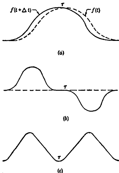
FIG. 12-30.—Pulse cancellation: (a) pulses, (b) residue, (c) rectified residues.
