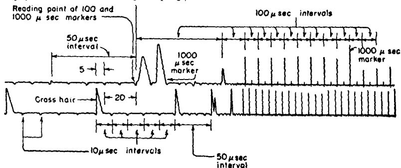
FIG. 7-7.—Display of fixed pulses on an exponential sweep (AN/APN-9). The time delay is measured between the pulse marked "cross hair" and the rise of the 50\text{-}\mu\text{sec} pulse on the upper trace. The "fine" scale reading is 20\ \text{plus}\ 5\ \mu\text{sec} as indicated. The integral number of 100\text{-}\mu\text{sec} intervals is counted with respect to the 1000\text{-}\mu\text{sec} marker and = zero \mu\text{sec} . The integral number of 1000\text{-}\mu\text{sec} markers shown on this sweep is 2, but in the actual indicator the number is determined by switching to a slower display and, for this particular case, corresponds to 6000\ \mu\text{sec} . The total reading is therefore 6025\ \mu\text{sec} .
