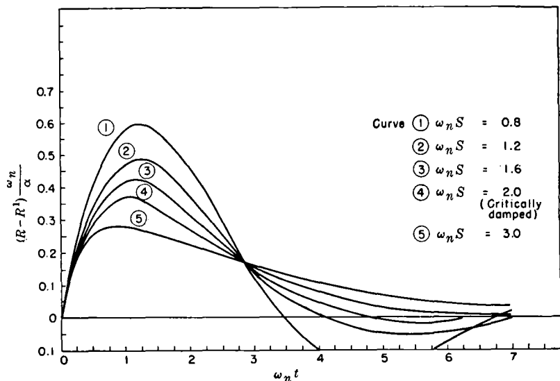
FIG. 8-5.—Behavior of R-R' in response to an instantaneous change \alpha in the value of dR/dt ( pR ) for various values of \omega_n^* . This is the response of a double-integrator system characterized by Eq. (19).
