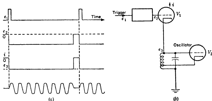
FIG. 12-18.—Pulsed oscillator.
