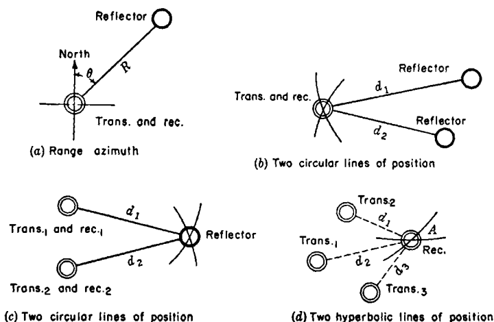
FIG. 2-20.—Some position-finding methods. The figure shows four basic position-finding methods. In (a) the position of the reflector is based on both the range and angle measurements made from a single transmitter and receiver. In (b) two circular lines of position are obtained from a pair of reflectors and a single transmitter-receiver. In (c) these lines are obtained from a pair of transmitter-receivers and a single reflector. In (d) two hyperbolic lines of position are obtained by a receiver at point A in combination with three transmitters and two receivers.
