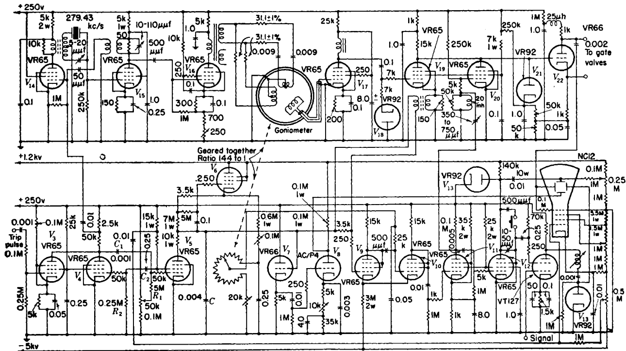
FIG. 7.42.—British CMH range circuit, type A presentation.
