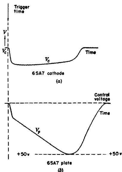
FIG. 5-9.—Phantastron waveforms.
