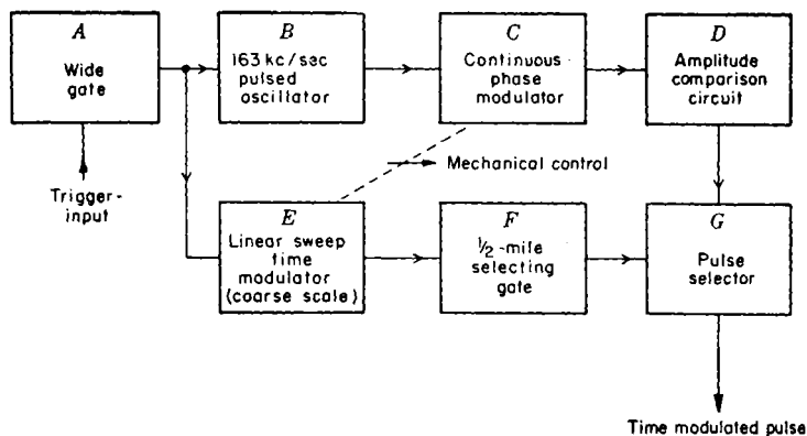
FIG. 6-8.—Block diagram of Precision Range Indicator.
