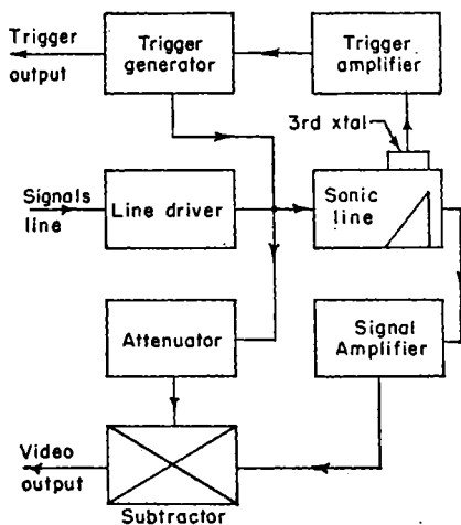
FIG. 12-35.—Three-crystal line.
