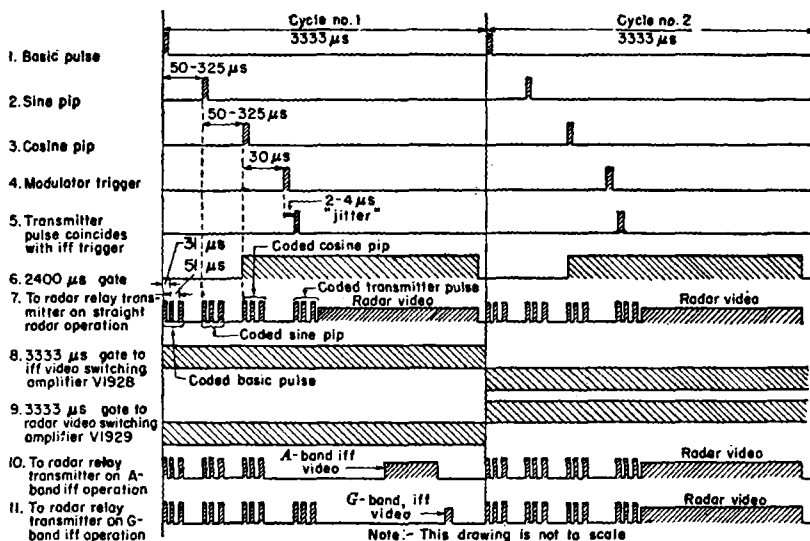
FIG. 11-7.—Synchronizer waveforms.
