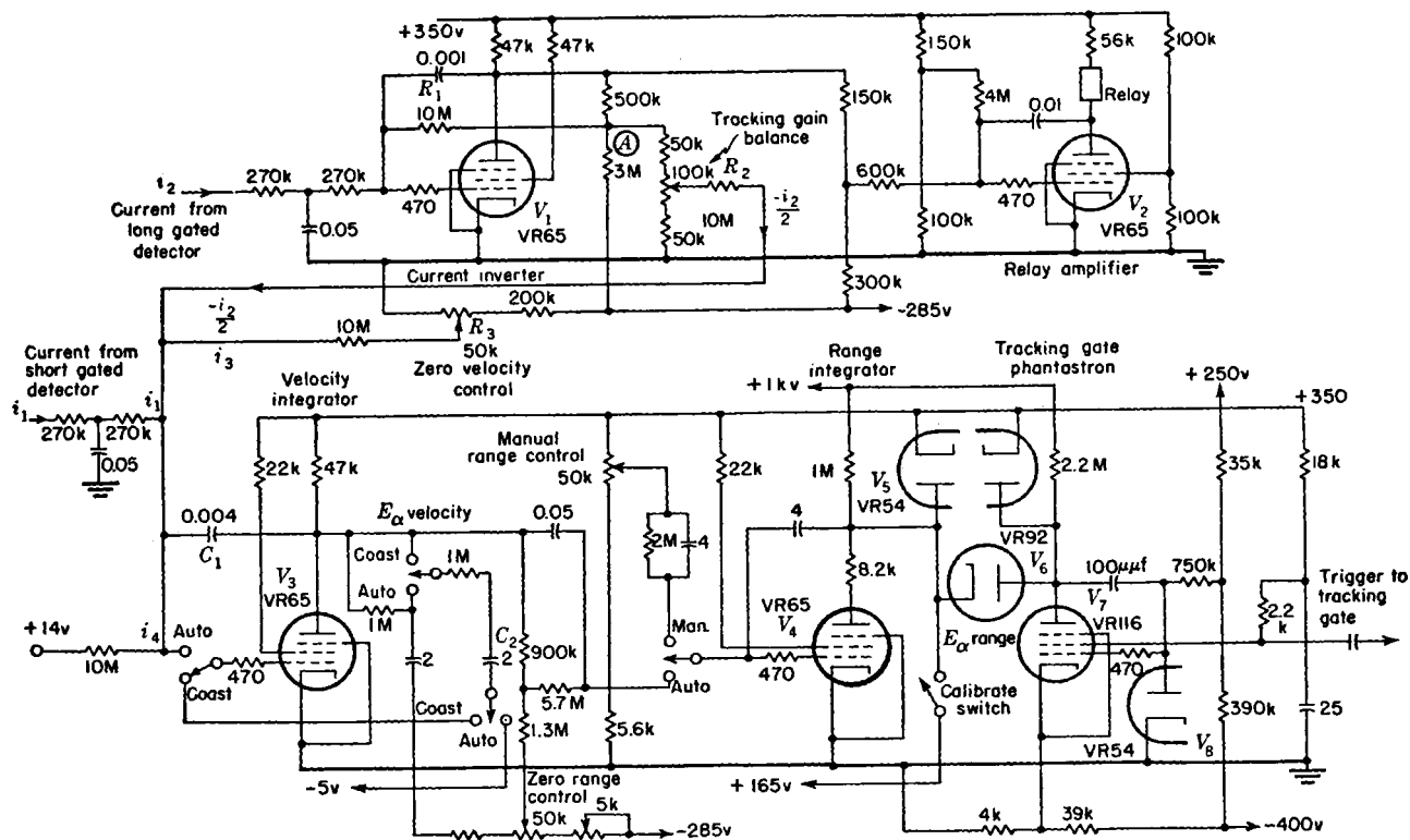
FIG. 9-14.—Oboe tracking-gate phantatron, and function unit, showing specially designed electrical integrators, and coast provisions.
