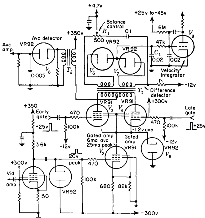
FIG. 8-32.—Time discriminator of British radar set.
