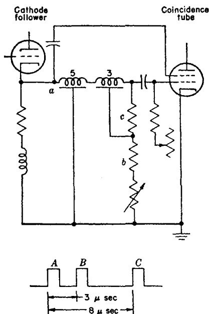
FIG. 11-11.—Decoding delay line.
