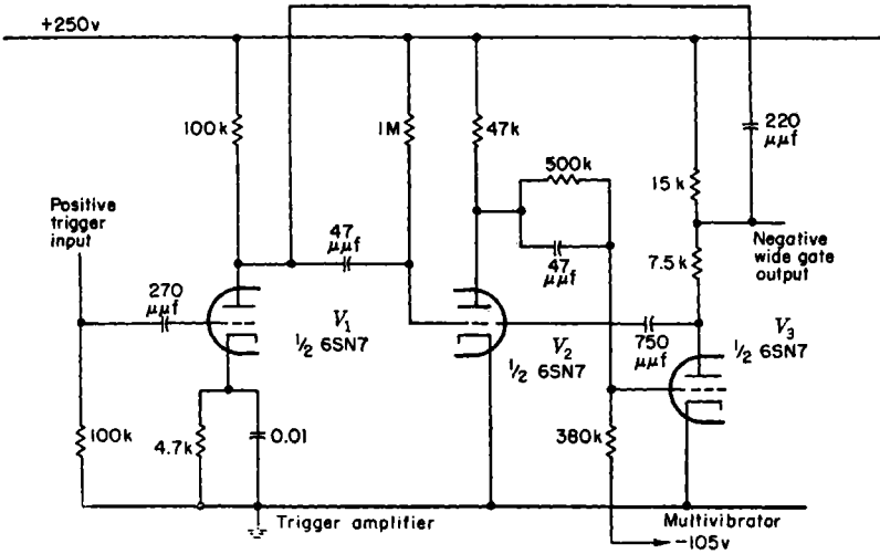
FIG. 6-10.—Wide-gate multivibrator of Precision Range Indicator.
