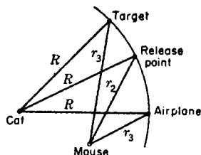
FIG. 9-8.—Geometry of Oboe blind bombing.
