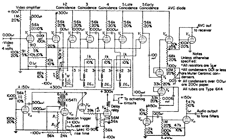
FIG. 10-9.—Decoder for remote control.
