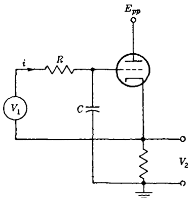
FIG. 8-22.—Bootstrap integrator.
