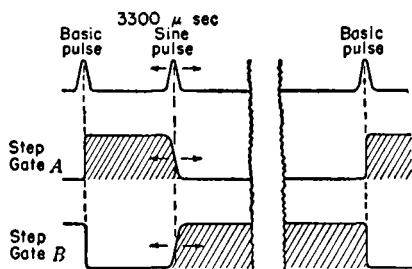
FIG. 11-13.—Timing diagram of sine-pulse step gates.
