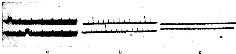
FIG. 7-6.—Time measurement by fixed pulses on a type A display (AN/APN-4). Three sweep speeds are required to resolve the time-difference reading between the upper and lower traces. In (a) the spacing of the pulses is 500\ \mu\text{sec} and a reading of 3500\ \mu\text{sec} is obtained. In (b) the spacing of the pulses is 50\ \mu\text{sec} and a reading of 350\ \mu\text{sec} is obtained. In (c) the spacing of the downward deflection is 50\ \mu\text{sec} and the small upward deflections, 10\ \mu\text{sec} . Interpolation gives a reading of 24\ \mu\text{sec} . The total reading is 3874\ \mu\text{sec} (Courtesy of McGraw-Hill Publishing Company.)
