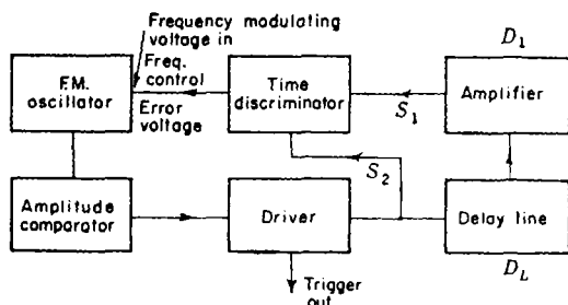
FIG. 12-37.—Electronic frequency tracking.
