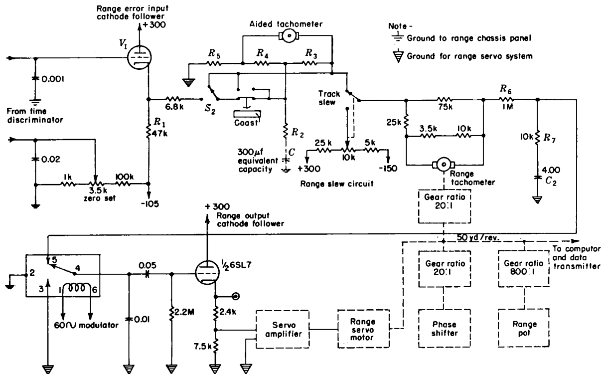
FIG. 9-18.—Function unit circuit complete except for 300 \mu condenser circuit of Fig. 9-17.
