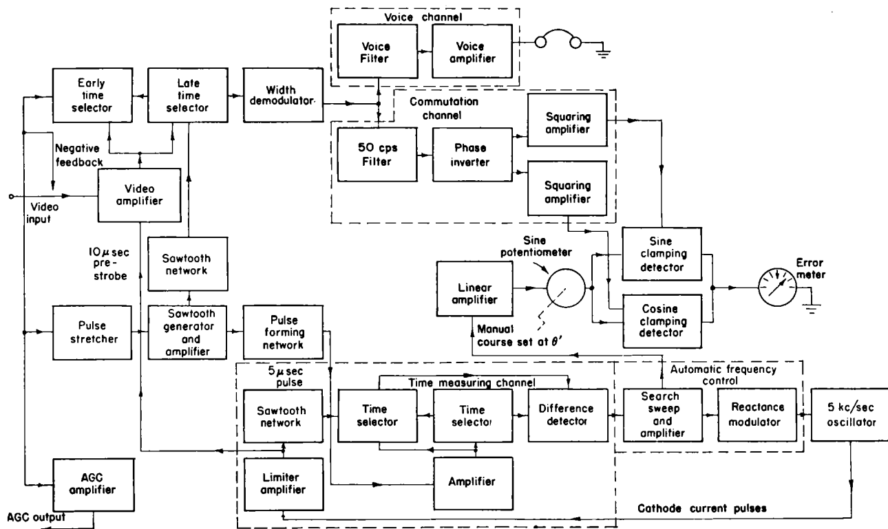
FIG. 10-13.—Block diagram of omnidirectional beacon demodulator.
