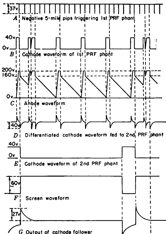
FIG. 4-32.—Waveforms of Oboe PRF divider.
