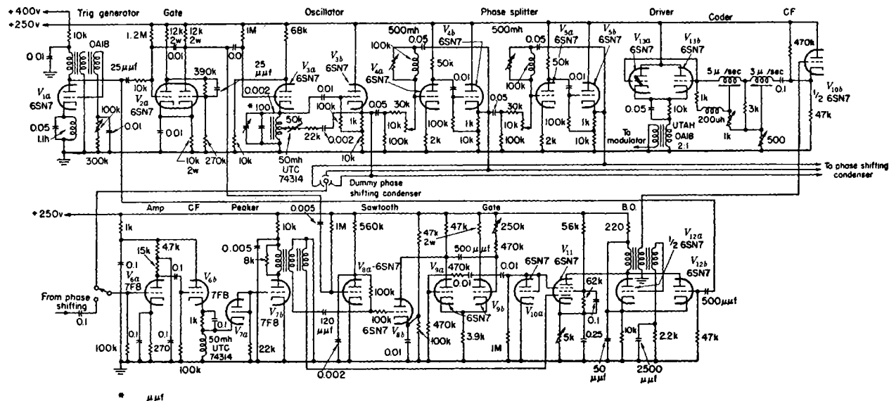
FIG. 11-21.—Synchronizer of phase-shifted pulse system.
